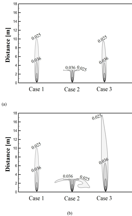
Fig. 4. Leakage distance for different crack positions at plane 1 and 2 (a) 10 s (b) 180 s
