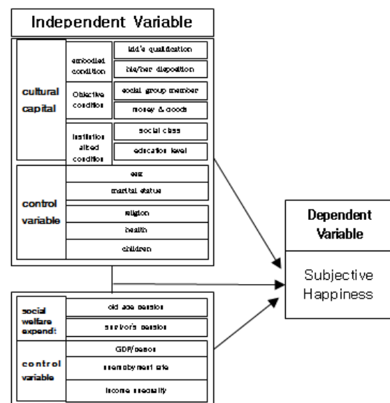
Fig. 2. Research model
