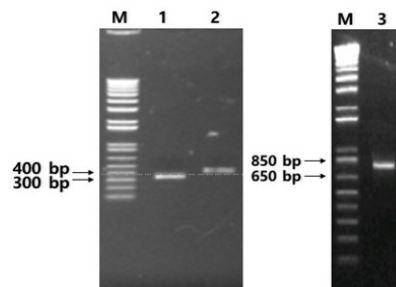
Fig. 1. PCR products of V H , V L , and scFv lane 1: V L , lane 2: V H , lane 3: scFv, M: DNA size standard 1kb ladder
