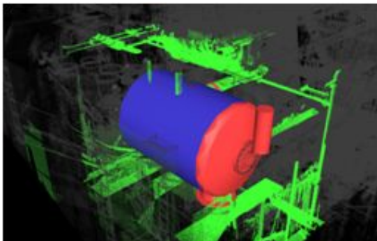
[Fig. 7] Crash Detect of Installation UV Type BWTS
