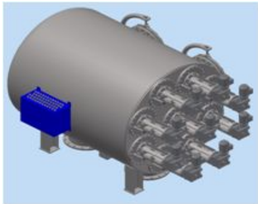
[Fig. 10] 3D Modeling for Filter of UV Type BWTS
