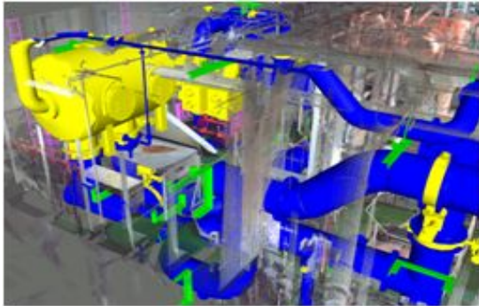
[Fig. 6] Installation Simulation of UV Type BWTS
