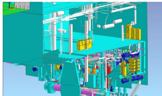
[Fig. 13] 3D Piping Modeling of Electrolysis Type BWTS
