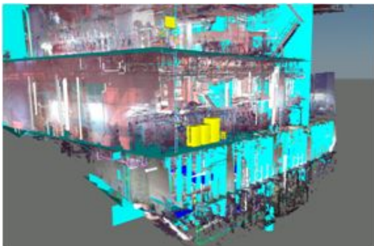
[Fig. 15] Harmonized 3D Modeling of Subject Vessel installed Electrolysis Type BWTS
