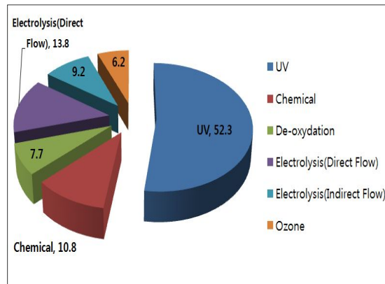
[Fig. 1] Distribution Ratio(%) by Treatment type for Type Approved BWTS
