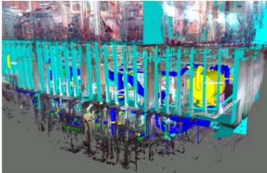
[Fig. 14] Harmonized 3D Modeling of Subject Vessel installed UV Type BWTS
