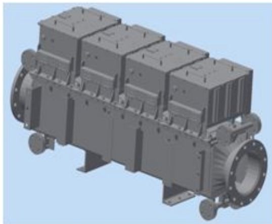
[Fig. 11] 3D Modeling for Module of Electrolysis Type BWTS
