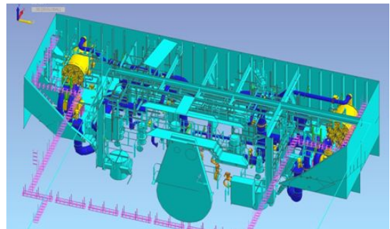
[Fig. 12] 3D Piping Modeling of UV Type BWTS
