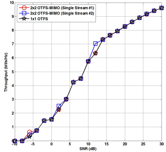
그림 14. 전송률 비교(1x1 OTFS, 2x2 OTFS-MIMO(#1, #2)) Fig. 14. Comparison of achievable rate(1x1 OTFS, 2x2 OTFS-MIMO(#1, #2)).
