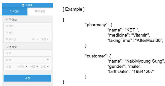
Fig. 7. Smartphone application for pharmacy (left) and a JSON format example (right)
