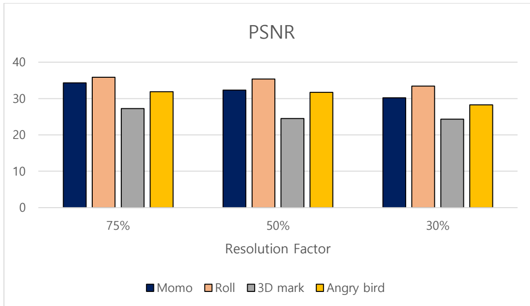
Fig. 16. Comparison of the PSNR for images which Game Tuner was applied
