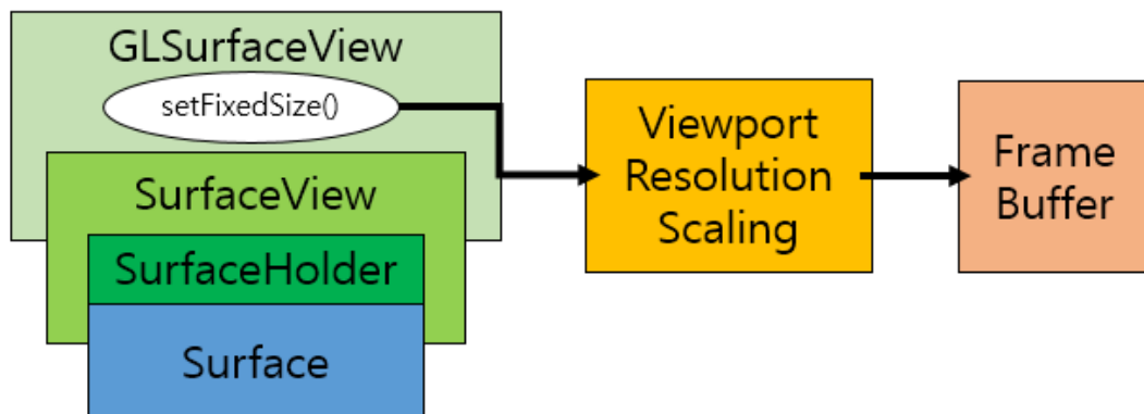
Fig. 7. Overview of VRS using the hardware scaler
