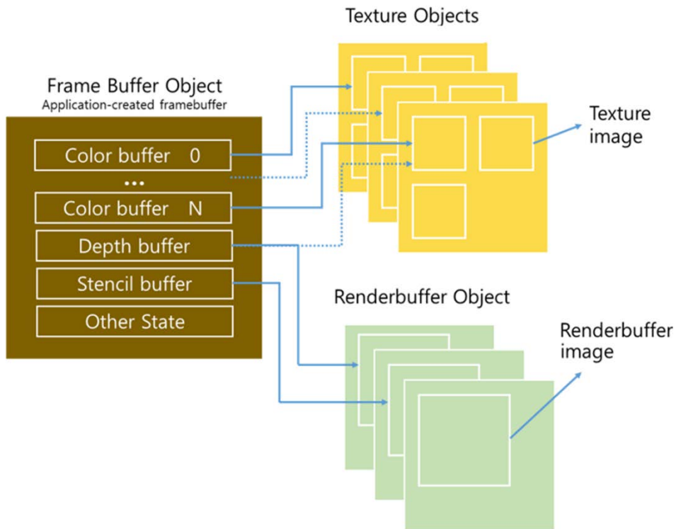
Fig. 6. FBO and its relationship with texture objects and renderbuffer objects [14]
