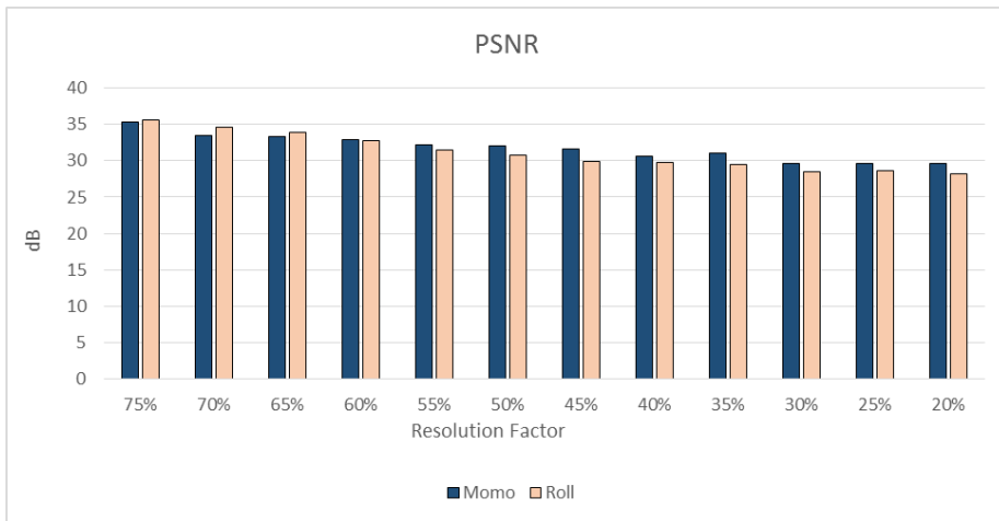
Fig. 14. Comparison of the PSNR between the Momo and Rolling Ball benchmark images
