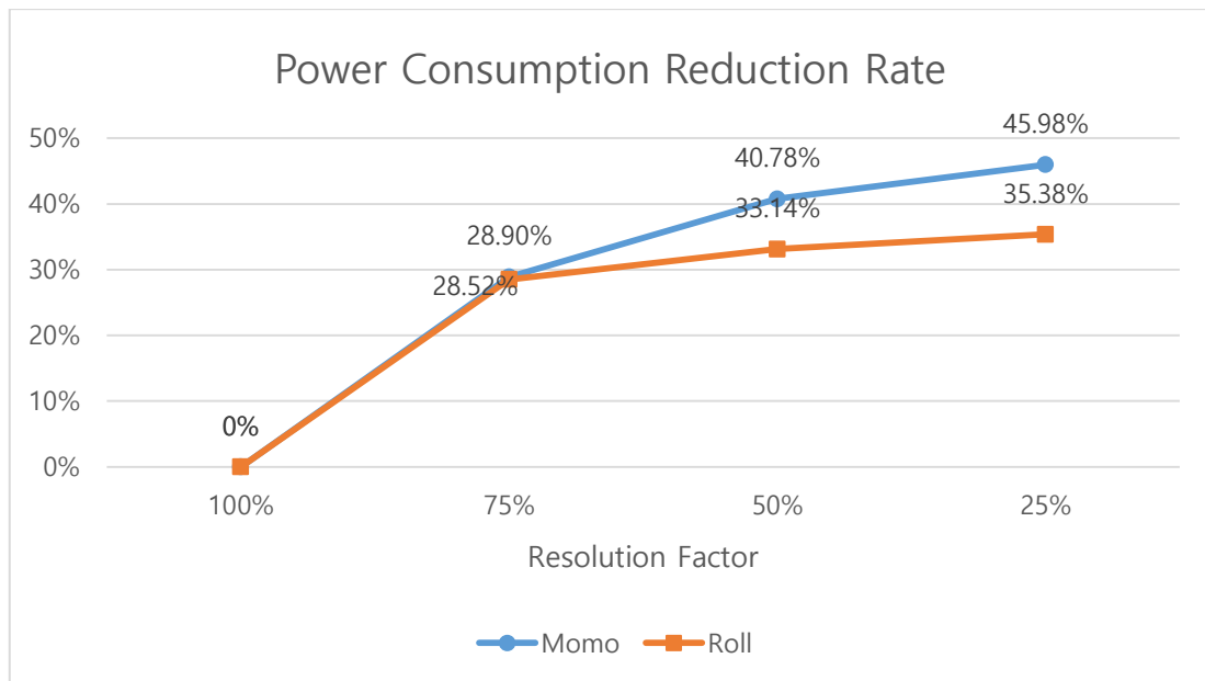
Fig. 17. Power Consumption Reduction Rate
