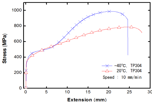
Fig. 6. Comparison of -40°C and 20°C in TP 304
