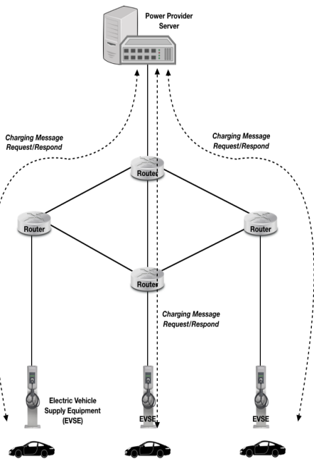
Fig. 1. The existing charging infrastructure
