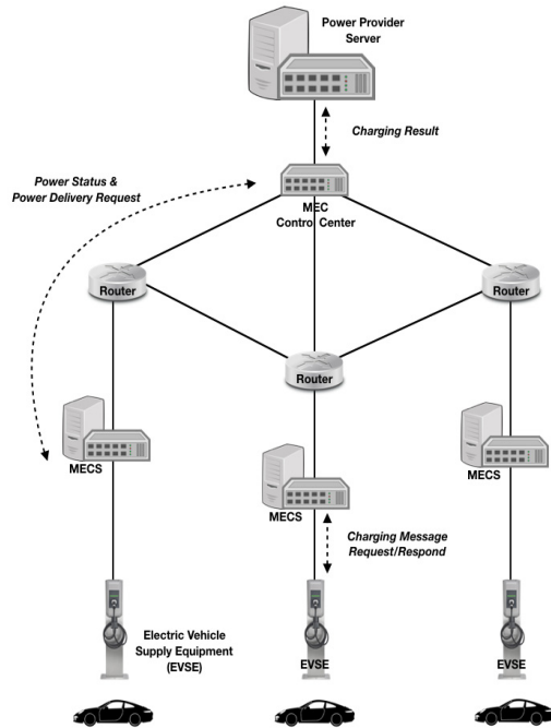
Fig. 2. The proposed charging infrastructure
