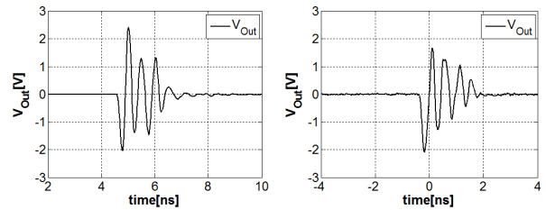
(a) 전압출력파형(시뮬레이션) (b) 전압출력파형(측정) (a) Voltage waveform(simulation) (b) Voltage waveform(measurement)
