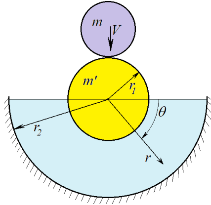
Fig. 3. Impact of two spheres studied by Joukowski (1884).
