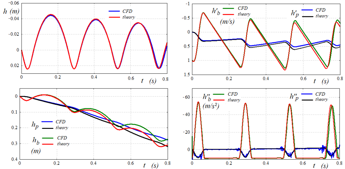
Fig. 5. Comparison of the theoretical and numerical results for the plate indentation h , displacements h_p and h_b , speeds h'_p and h'_b and the accelerations h''_p and h''_b of the plate and the body, respectively, as functions of time t .
