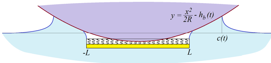
Fig. 6. Impact of a large body onto a floating plate with pile-up effect.
