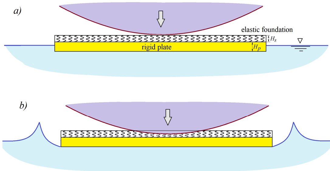
Fig. 4. Impact on a floating plate with an elastic layer on the top of it before the interaction (a) and during the interaction (b).
