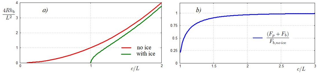
Fig. 7. Non-dimensional penetration depth of the body (a) and the non-dimensional hydrodynamic force (b) as functions of the scaled length, c/l , of the wetted part of the body surface.
