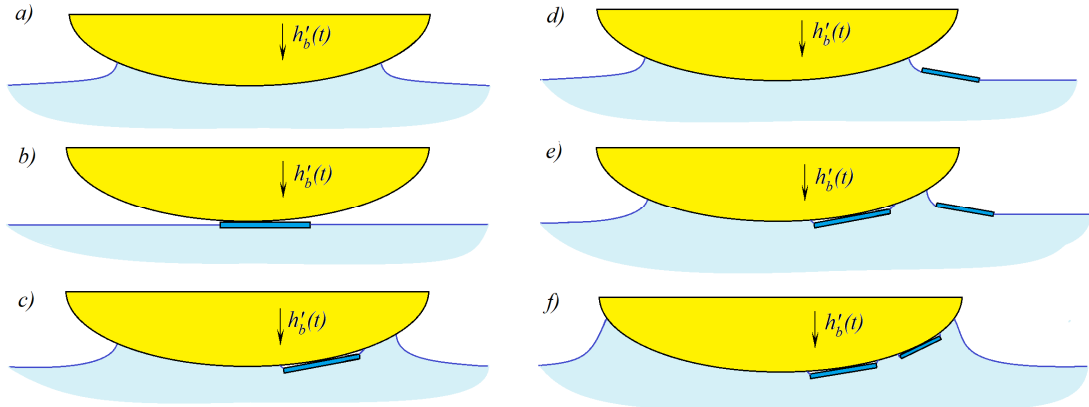
Fig. 1. Two-dimensional slamming for open water (a), with ice floe (b), which is attached to the body surface later on (c), with an ice floe near the impact region (d), several floes under and near the body surface (e) and floes on the body surface (f).
