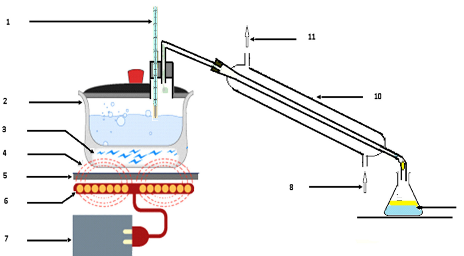
1- Thermometer; 2- Saucepan; 3- Induced current; 4- Magnetic field; 5- Glass-ceramic plate; 6- Induced coils (electromagnet); 7- Power supply; 8- Water inlet; 9- Distillate; 10- Refrigerant; 11- Water outlet.
