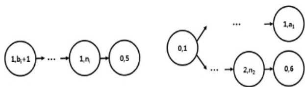
Fig. 7. The precedence graphs for Subproblems 1 and 2 reduced from Subproblem 5
