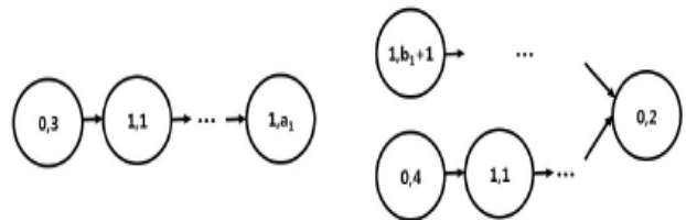
Fig. 6. The precedence graphs for Subproblem 1 and 3 reduced from Subproblem 5
