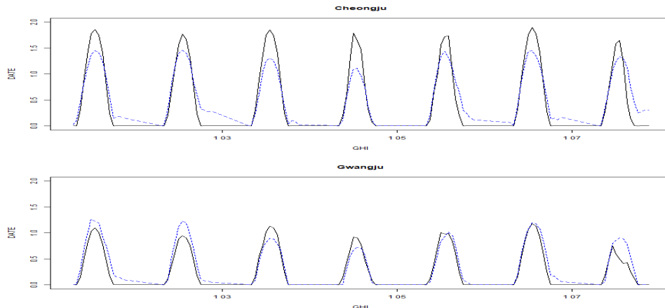
Figure 3.5. Result of forecasting 7-Days ahead, ARIMAX model. ARIMAX = auto-regressive integrated moving average with eXogenous variable.
