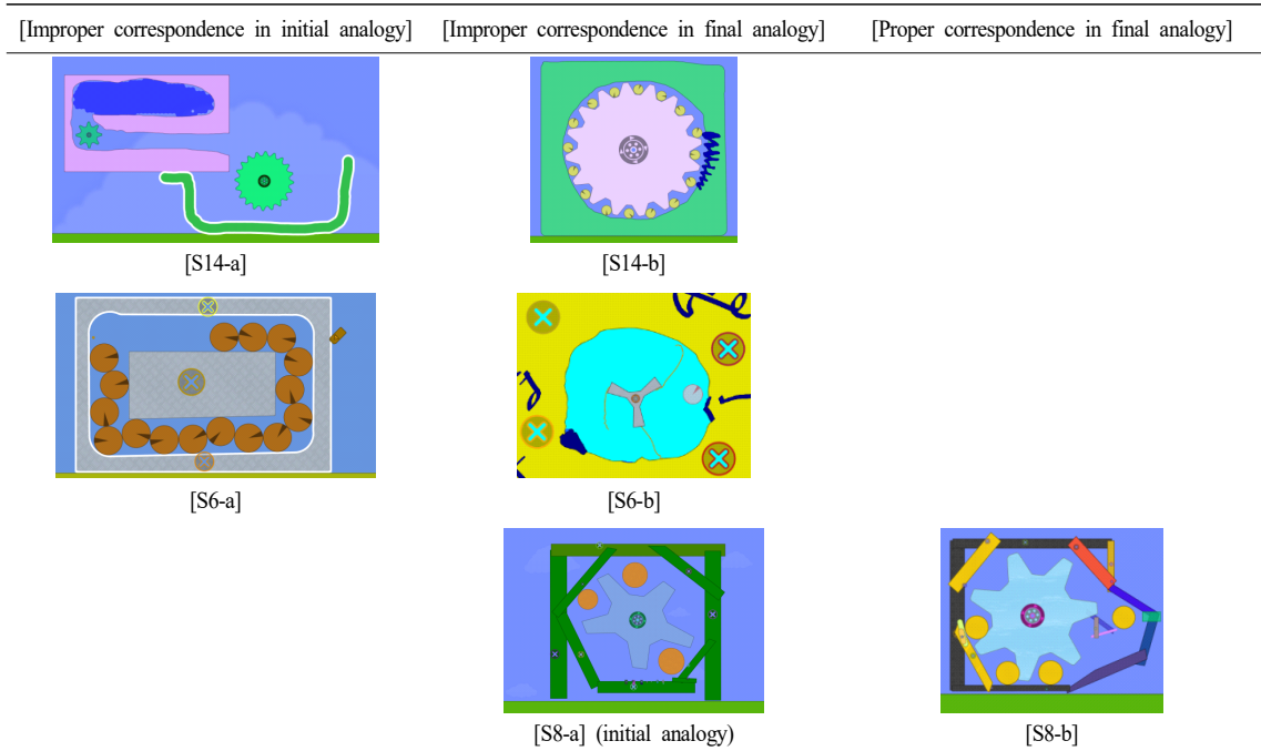
Fig. 7. Changes for constant speed of the circulating free electrons represented by the circular particles.
