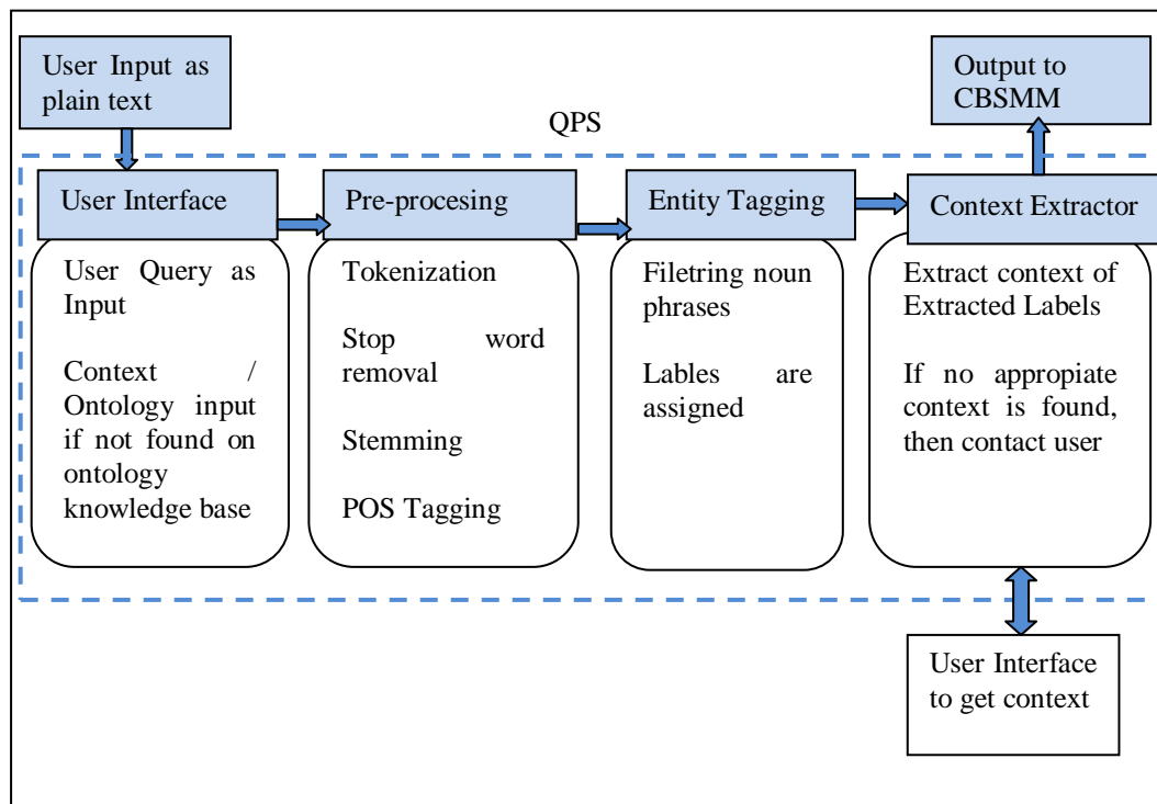
Fig. 2. QPS Pipeline
