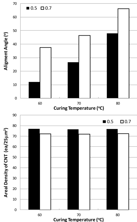
Fig. 6. Alignment and areal density of MWCNTs of MWCNT-PDMS microstructures w.r.t the curing temperature and relative degree of cure
