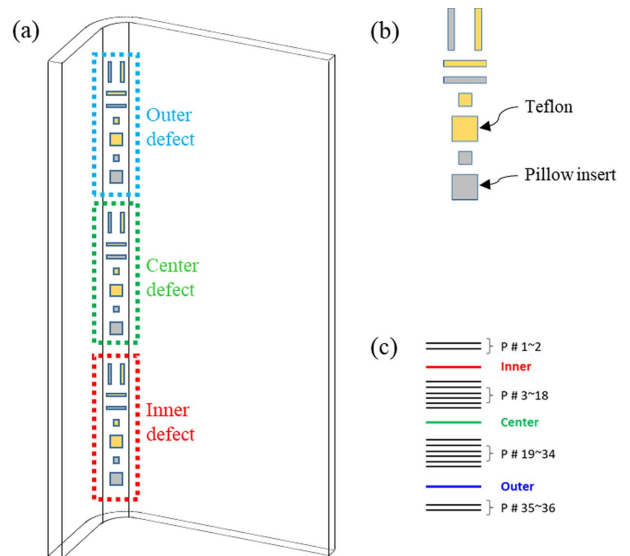
Fig. 3. L-shaped specimen: (a) specimen overview, (b) defect type and shape, and (c) stacking sequence
