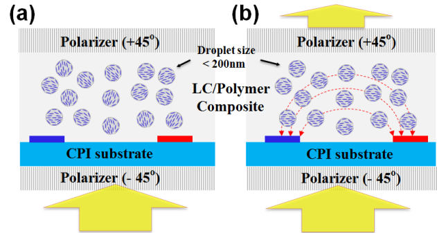
FIG. 3. Schematic of the flexible optically isotropic liquid crystals (a) at voltage-off and (b) voltage-on states.
