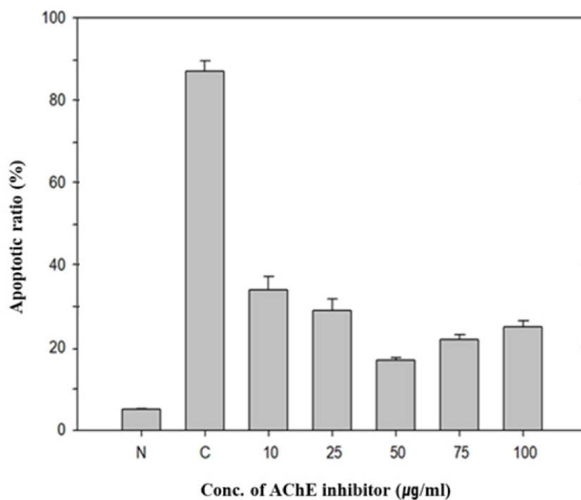
Fig.3. Apoptotic ratio on PC12 nerve cell of the partial purified acetylcholinesterase(AChE) inhibitor. N, CT105 not treated; C, CT105 treated
