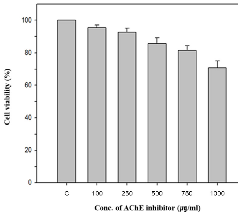
Fig. 2. Cell viability on PC12 nerve cell of the partial purified acetylcholinesterase(AChE) inhibitor. C, AChE inhibitor not treated
