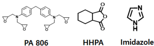
Fig. 7. Molecular structure of PA 806 + HHPA + Imidazole
