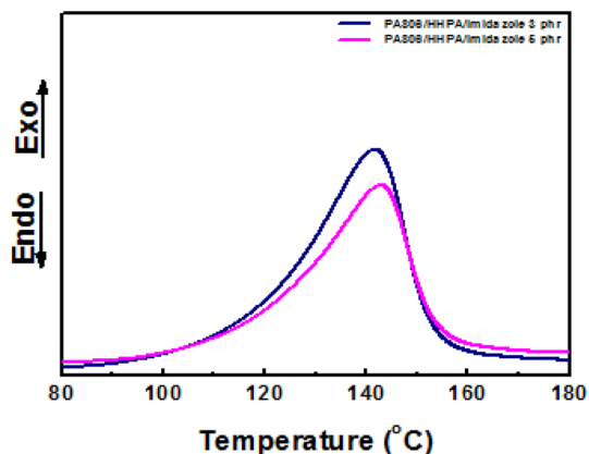
Fig. 8. DSC curve for 1 st heating cycle of PA 806 + HHPA + Imidazole
