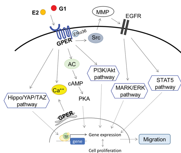
Fig. 1. Proposed mechanism of GPER in cancer cells. AC, adenylyl cyclase; PKA, protein kinase A; MMP, matrix metalloproteinase; EGFR, epithelial growth factor receptor; TF, transcriptional factor.
