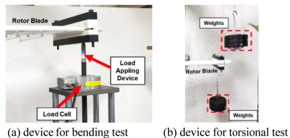
Fig. 3. Load applying devices
