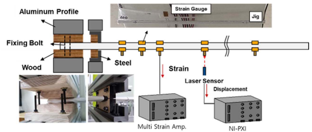
Fig. 2. Schematic representation of test apparatus
