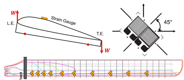
Fig. 9. Strain gauges installation for torsional test
