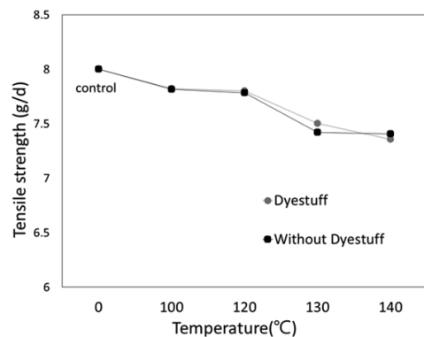
Figure 4. The variations of the tensile strength of SC-CO 2 dyed PET filaments under different dyeing temperature condition.
