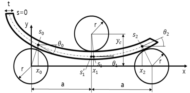
Fig. 6 Geometric relationship between rollers and workpiece
