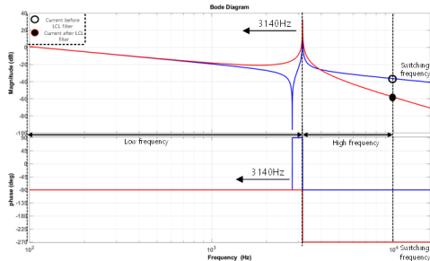
Fig. 2. LCL filter transfer function board diagram
