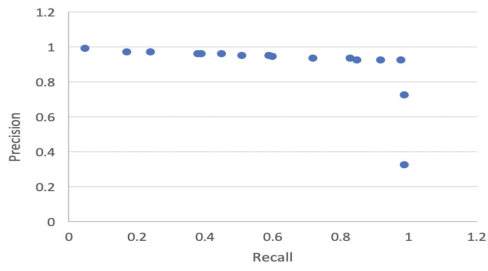
Fig. 8. Precision-recall curve
