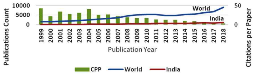
Fig. 1. Artificial Neural Networks Research Growth- Global Vs India 1999-2018
