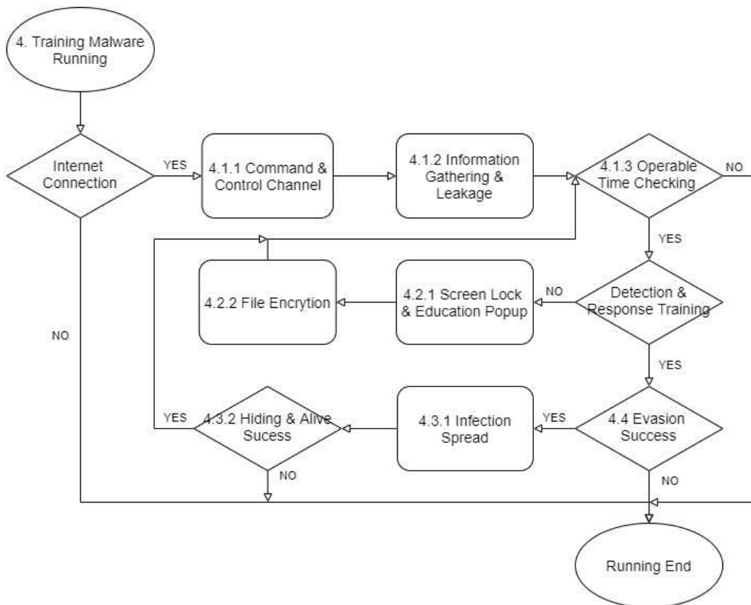
Fig. 2. Training Malware Running Flow
