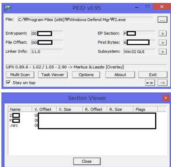
Fig. 3. Training Malware Custom Packing
