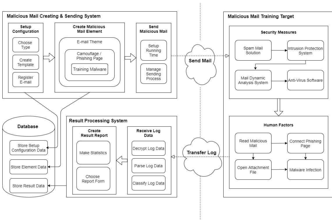
Fig. 1. Malicious Mail Training Model Design
