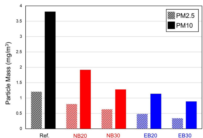
Figure 6. Wear particulate matters generated by rubber compounds abrasion.
