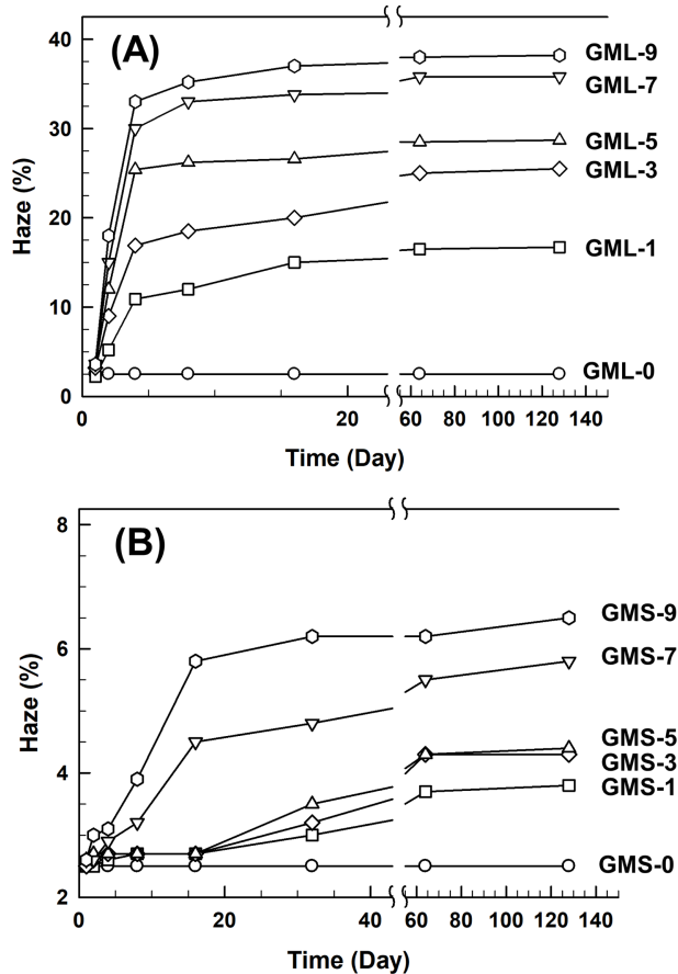
Figure 6. The haze of rPP compound film according to antifogging agent content and aging time: (A) GML and (B) GMS.
