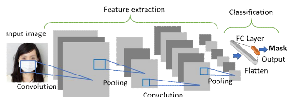
Fig. 1. CNN architecture
