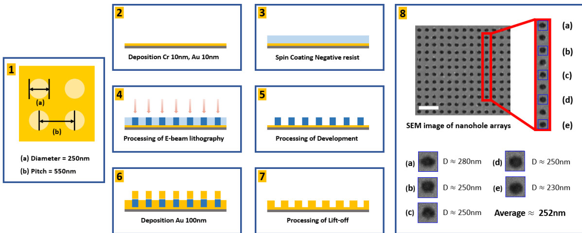
Fig. 2. Process of fabricating the subwavelength nano hole arrays. (1) The image of nanohole array patten; diameter 250 nm and pitch 550 nm, (2) deposition of Cr 10 nm and Au 10 nm on BK7, (3) spin coating of negative E-beam resist, (4) processing of E-beam lithography, (5) processing of development, (6) deposition of Au 100 nm, (7) processing of lift-off, and (8) the SEM image of nanohole arrays. The scale bar is 1 μm and the hole diameter is calculated by using the SEM.
