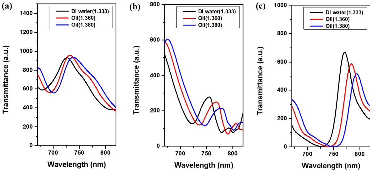
Fig. 5. Simulation results of transmission spectra of (a) focused beam (10×), (b) focused beam (4×), and (c) collimated beam when using DI water; n = 1.333 and the refractive index matching oil; n = 1.360 and 1.380 .
