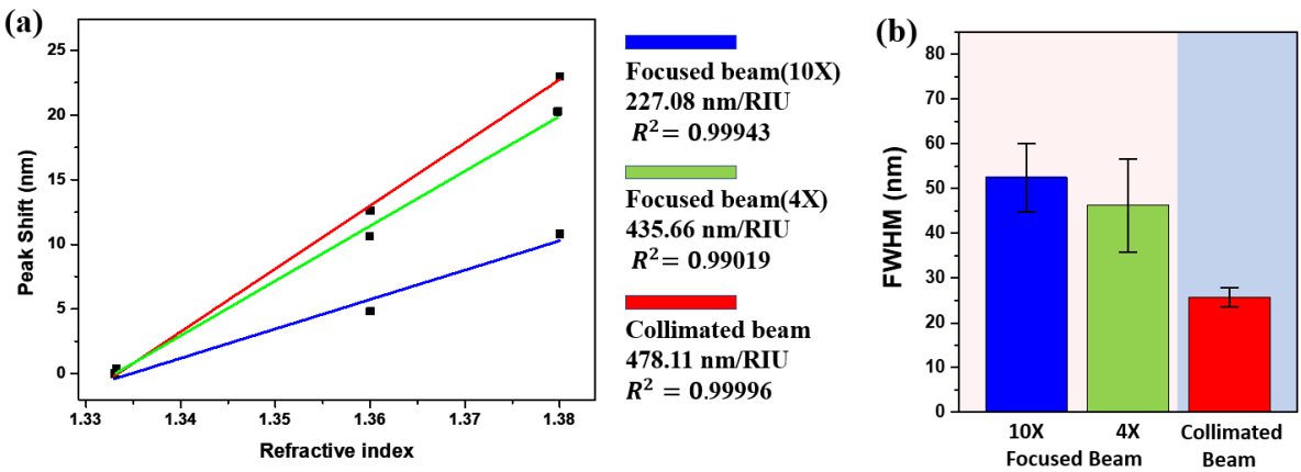
Fig. 6. Simulation results. (a) Calibration plot of sensitivity. (b) Calculated FWHM (blue line, focused beam (10×); green line, focused beam (4×); red line, collimated beam).
