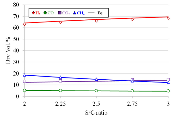
Fig. 7. Reforming gas composition measurement result according to SCR change
