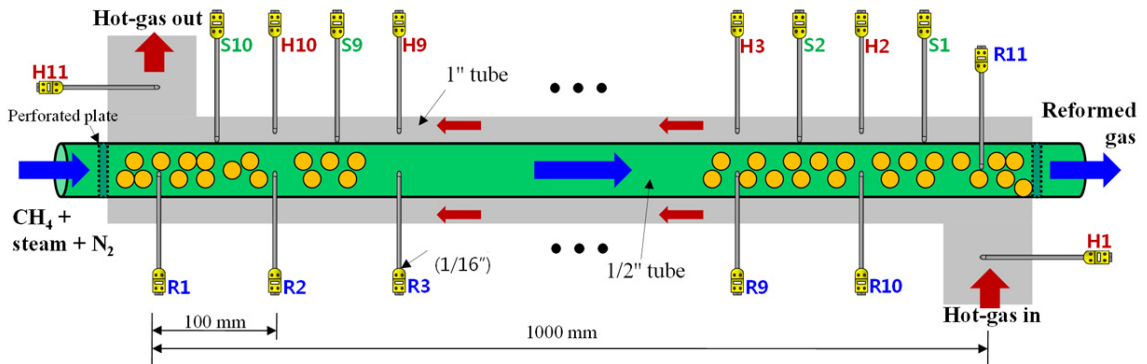
Fig. 2. Configuration of catalyst reactor
