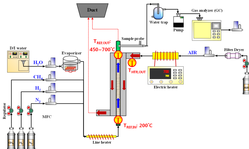
Fig. 3. Configuration of catalyst characteristic experiment
