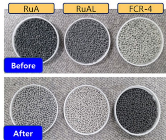
Fig. 1. Commercial catalysts used in the experiment
