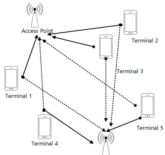
Fig. 1. System Model
