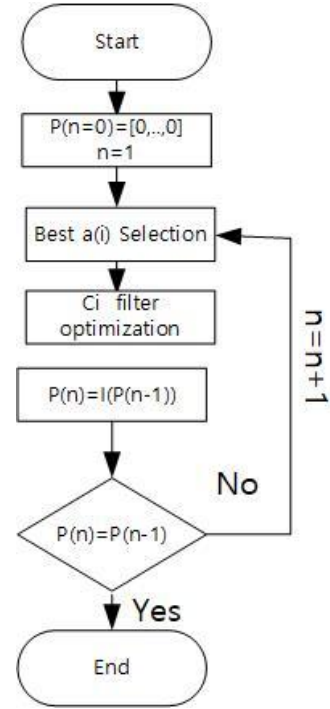
Fig. 2. Proposed Algorithm
