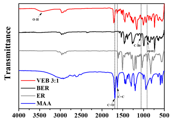
Fig. 2. FTIR spectra of starting materials and product
