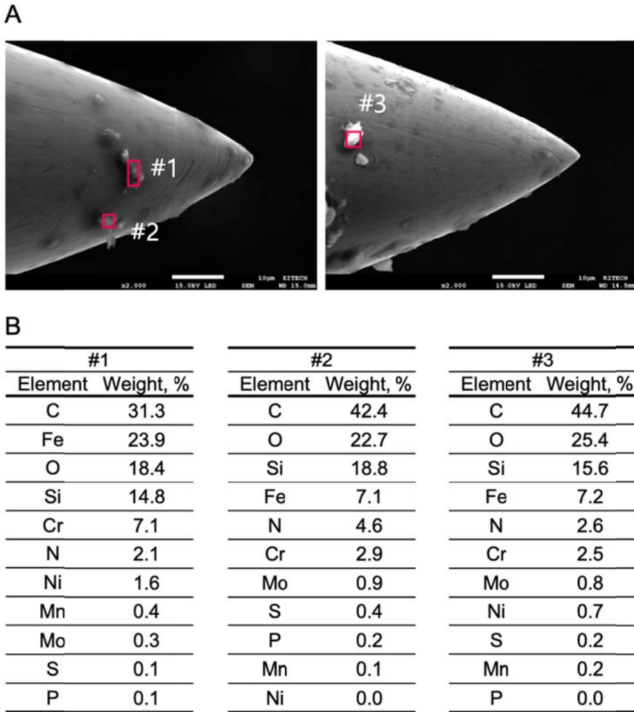
Figure 3. EDS analysis of foreign materials of acupuncture needle tips: (A) selected points on SEM images, (B) weight ratio of selected elements at each point. SEM, scanning electron microscopy; EDS, energy-dispersive X-ray spectroscopy.
