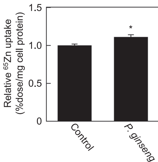
Fig. 2. P. ginseng extract induces zinc uptake in Hepa cells. Hepa cells were incubated for 24 h in normal medium (control) in the absence or presence of 1000 µg/mL P. ginseng extract. Zinc uptake rates for 20 min were calculated and normalized to protein concentrations. * P < 0.05 , significantly different from control. Each bar represents the mean \pm S.D. (n = 3).
