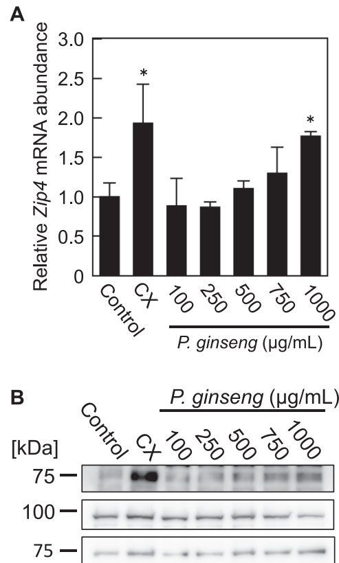
Fig. 3. Induction of Zip4 expression by P. ginseng extract in a concentration-dependent manner. (A) Total RNA isolated from Hepa cells cultured under the indicated conditions for 24 h was subjected to RT-qPCR. * P < 0.05 , significantly different from control. Each bar represents the mean \pm S.D. (n = 3). (B) Membrane proteins (18 µg) from Hepa cells treated with the indicated concentrations of P. ginseng extract for 24 h were separated by 10% SDS-PAGE. The expression of Zip4, Na,K-ATPase, or GRP78 was detected with specific antibodies.
