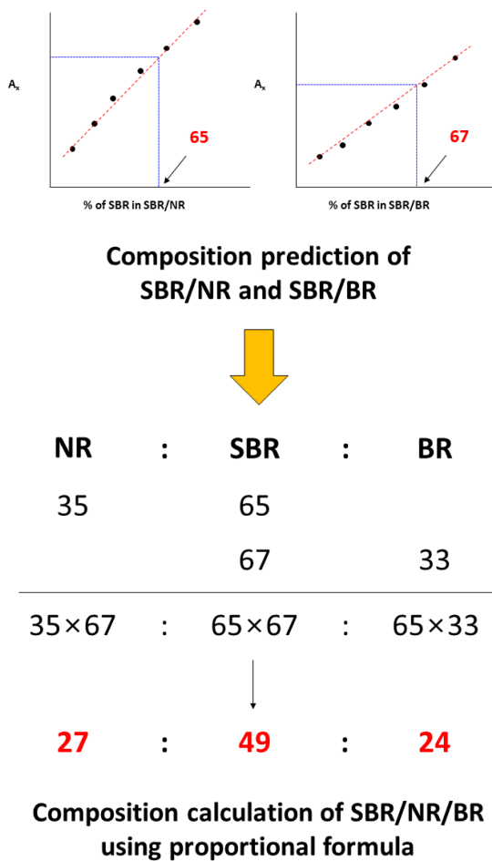
Figure 5. Composition prediction process of SBR/NR/BR (50/25/25).
