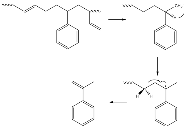
Scheme 2. Pyrolysis mechanism for formation of 2-phenylpropene (2-PP) from butadiene-styrene heterosequence of SBR.
