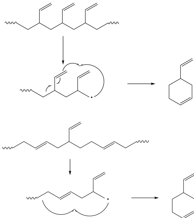
Scheme 1. Pyrolysis mechanism for formation of 4-vinylcyclohexene (4-VCH) from butadiene sequence.
