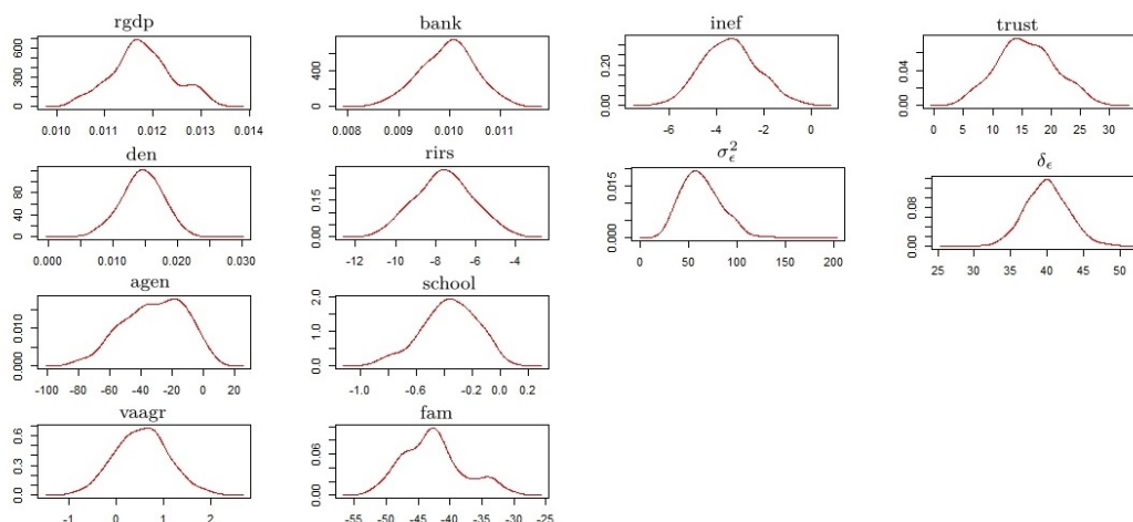
Figure 4: Markov chain density for parameters under random model of the Italian non-life insurance data.
