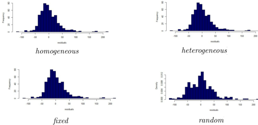
Figure 2: Data on non-life insurance consumption in Italy. Histogram of residuals for each type of spatial effect after fitting the multivariate normal distribution, for each space.
