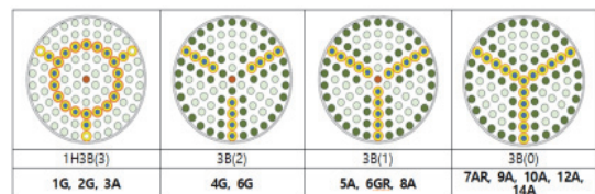
* 1H3B - 1Hub and 3 Baffle Injectors, 3B - 3 Baffle Injectors ** The number in parentheses is the starting point number of the baffle injector lines installed outward from the center.
