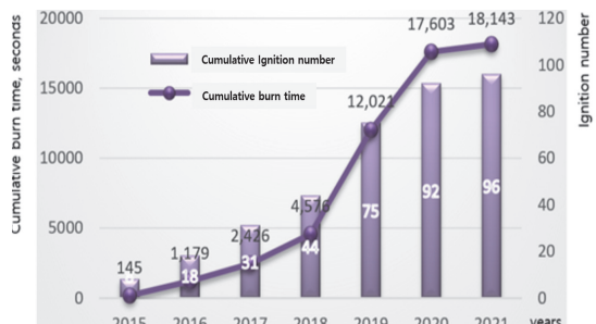
Fig. 10 Combustion test status of the KSLV-II upper stage engines.
