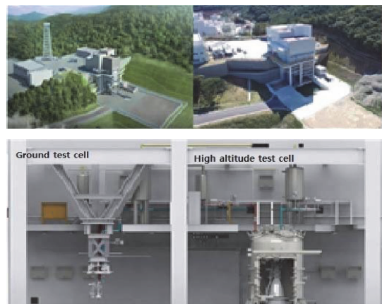
Fig. 6 Upper stage engine test facilities[7].
