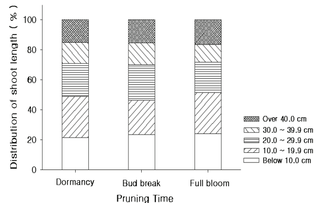
Fig 1. Distribution of shoot length of 'Fuji'/M.9 apple trees in the treating year as affected by delaying winter pruning.
