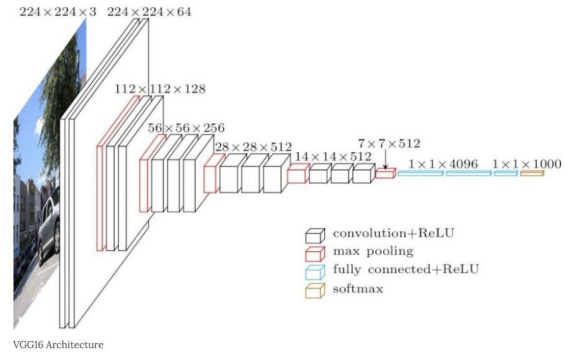
Fig. 2. VGG16 Architecture [11]
