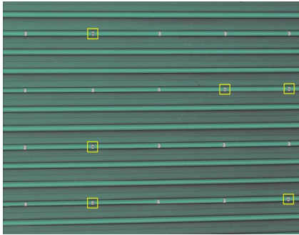
Fig. 12. Result Image
