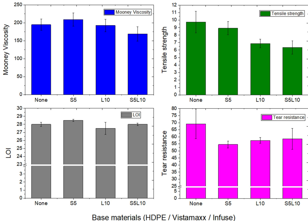
Fig. 5. Comparison of mechanical properties of flame retardant-added thermoplastic composites mixed with various types of base polymers
