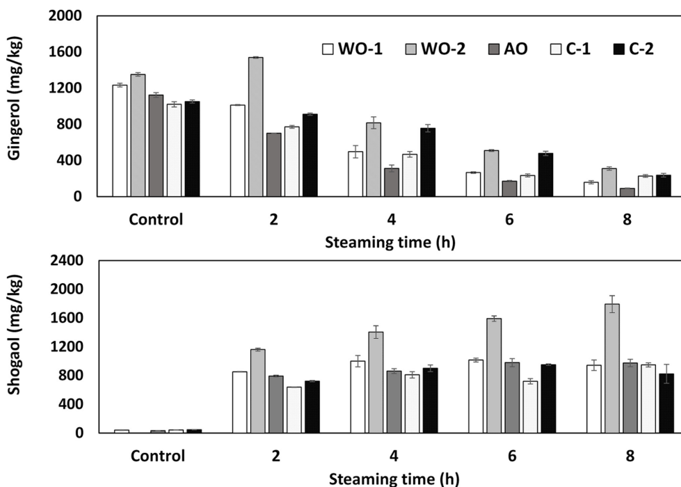
Fig. 2. Content of total gingerols and shogaols according to the steaming time.
