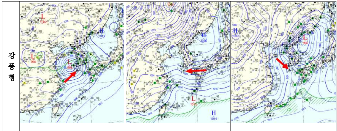
Fig. 4. Pressure pattern associated with strong wind speed
