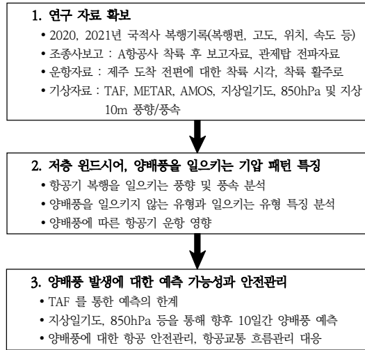
Fig. 3. Research workflow
