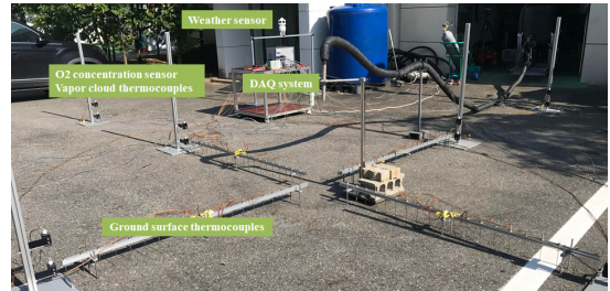
Fig. 4. Photo of measuring sensors
