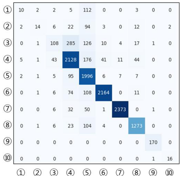
Fig. 3. Confusion Matrix of Multi-class Classification(BERT)
