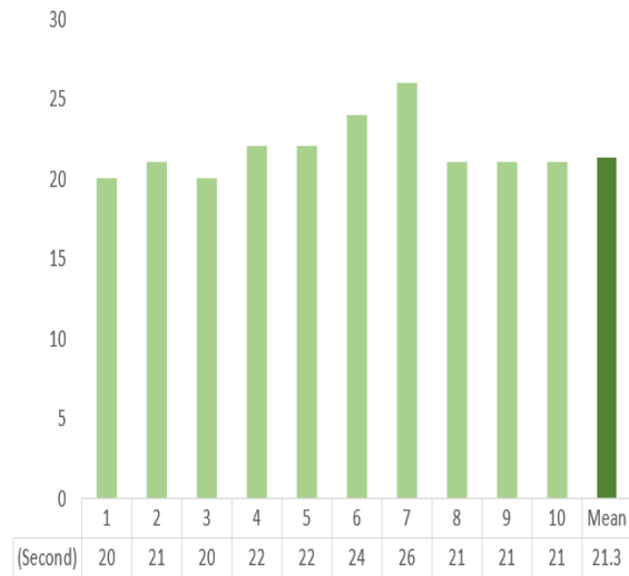
Fig. 10. Service response time
