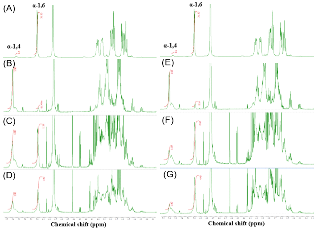
Fig. 4. ^1\text{H-NMR} spectroscopy of Gluconobacter oxydans culture media added with maltodextrin and rice hydrolysate. (A), dextran ( \alpha -1,6 linkage); (B), maltodextrin media 0 h; (C), maltodextrin culture media 12 h; (D), maltodextrin culture media 72 h; (E), rice hydrolysate media 0 h; (F), rice hydrolysate culture media 12 h; (G), rice hydrolysate culture media 72 h.
