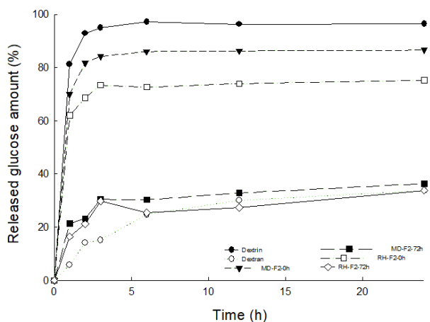
Fig. 5. Glucose generation by mammalian mucosal \alpha -glucosidases of Gluconobacter oxydans culture media added with maltodextrin and rice hydrolysate. Symbols: ●, dextrin; ○, dextran (positive control); ▼, maltodextrin media 0 h; ■, maltodextrin culture media 72 h; □, rice hydrolysate media 0 h; ◇, rice hydrolysate culture media 72 h.
